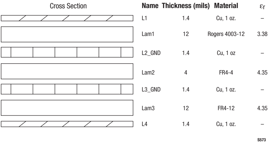
Figure 15. Layer Detail Physical Characteristics
